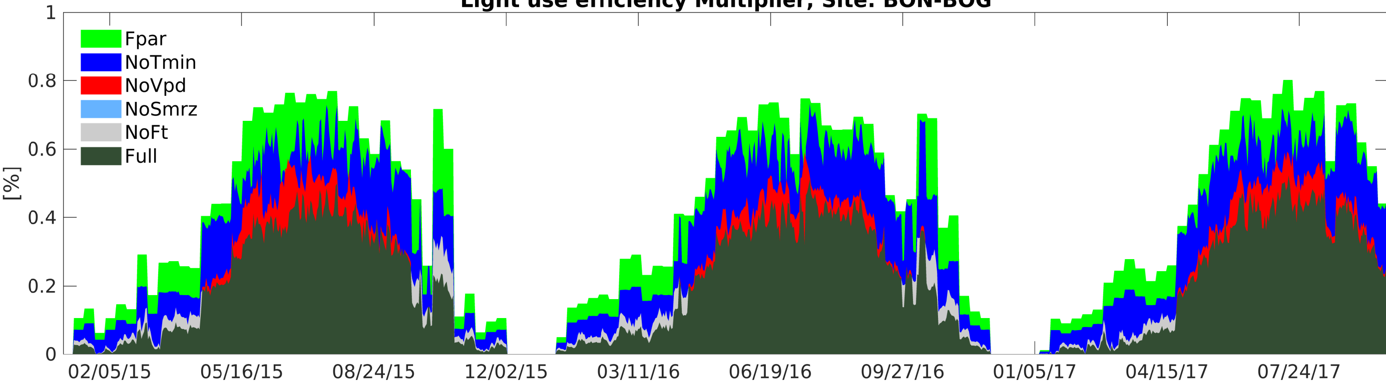
Light use efficiency Multiplier; Site: BON-BOG
