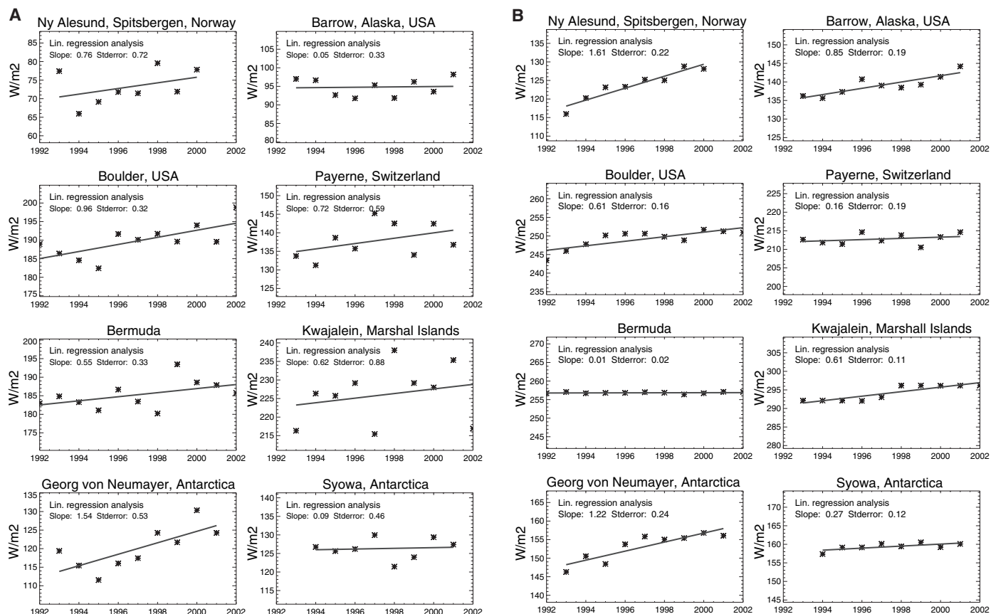
Fig. 2. Time series of annual mean surface solar radiation measured at worldwide distributed sites from BSRN. Shown are the eight longest records from BSRN covering the period 1992 to 2002 for (A) all-sky
